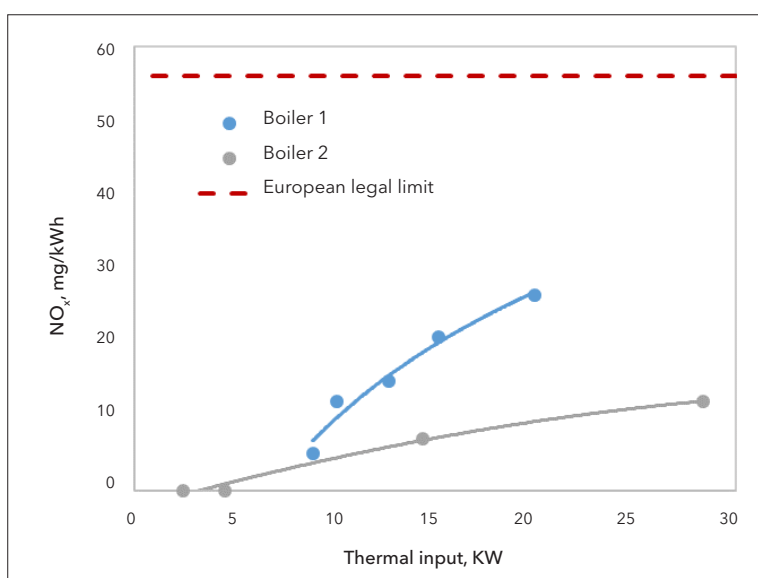
Figure 4 - Left: DNV GL/Gasterra (boiler 1) and Bekaert (boiler 2) condensing boilers in Rozenburg demonstration Right: NO x emission measured in hydrogen boiler 1 & 2 at different thermal loads
