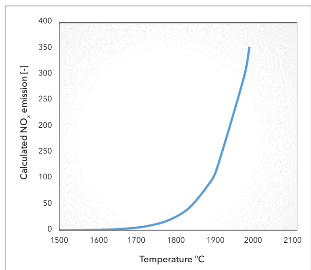
Figure 3: Calculated thermal NO formation as function temperature
